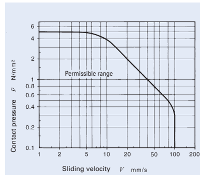
Fig. 2 pV diagram of lubrication type PILLOBALLS
