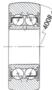
LD5800 (Spherical O.D. 400R)
