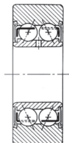
LD5700 (Cylindrical O.D.)
