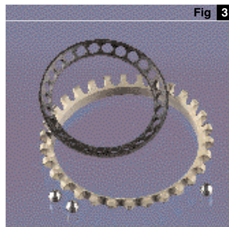
Cages for double direction angular contact thrust ball bearings
