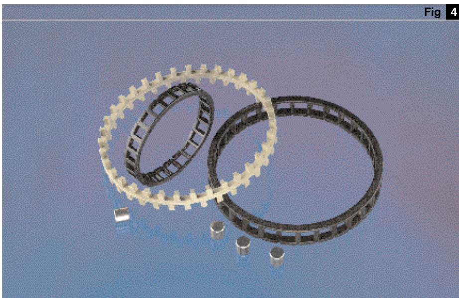
Cages for double row cylindrical roller bearings
